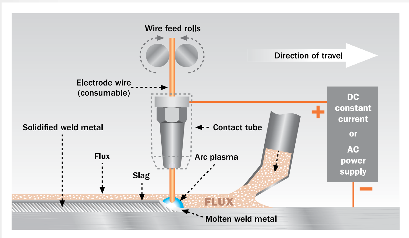
Single-wire Submerged Arc welding
