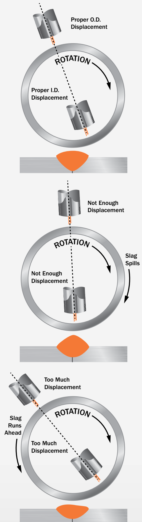
Figure 1 — Torch placement for circumferential SAW.
