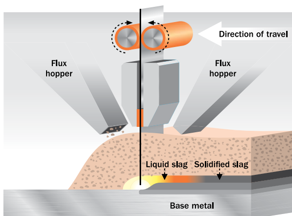
SAW strip cladding
