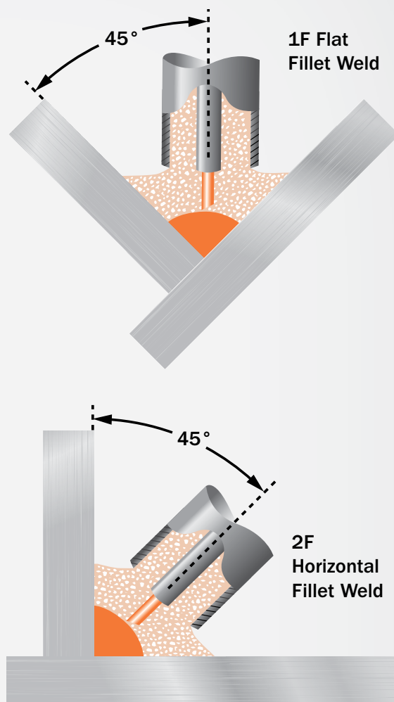
Figure 2 — Torch placement for SAW fillet welds on T-joints.
