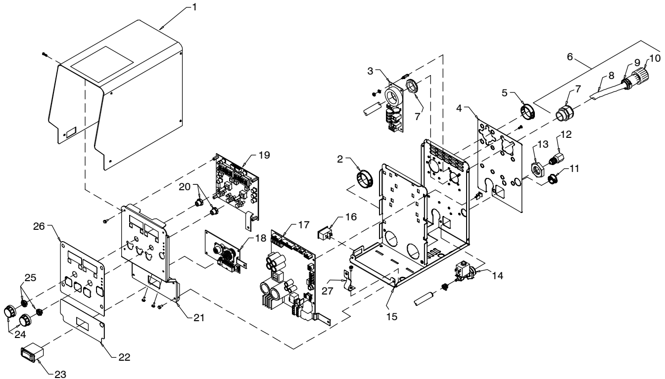
Figure 1-2. Control Box
