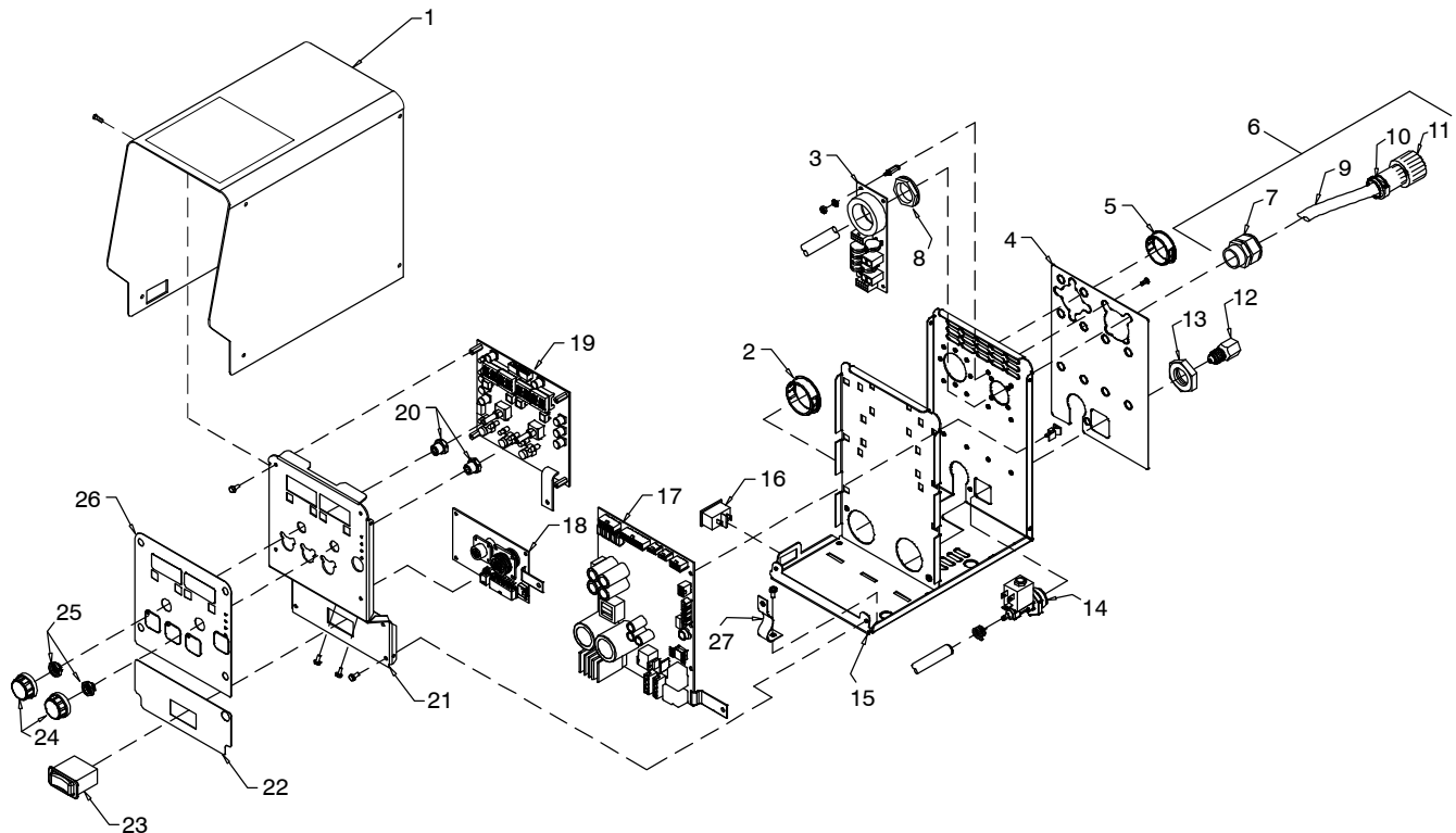
Figure 3-2. Control Box
