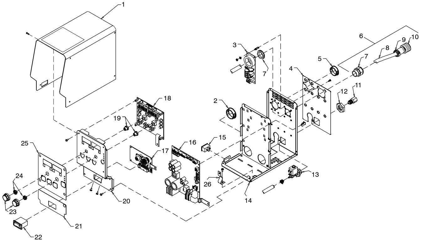
Figure 2-2. Control Box
