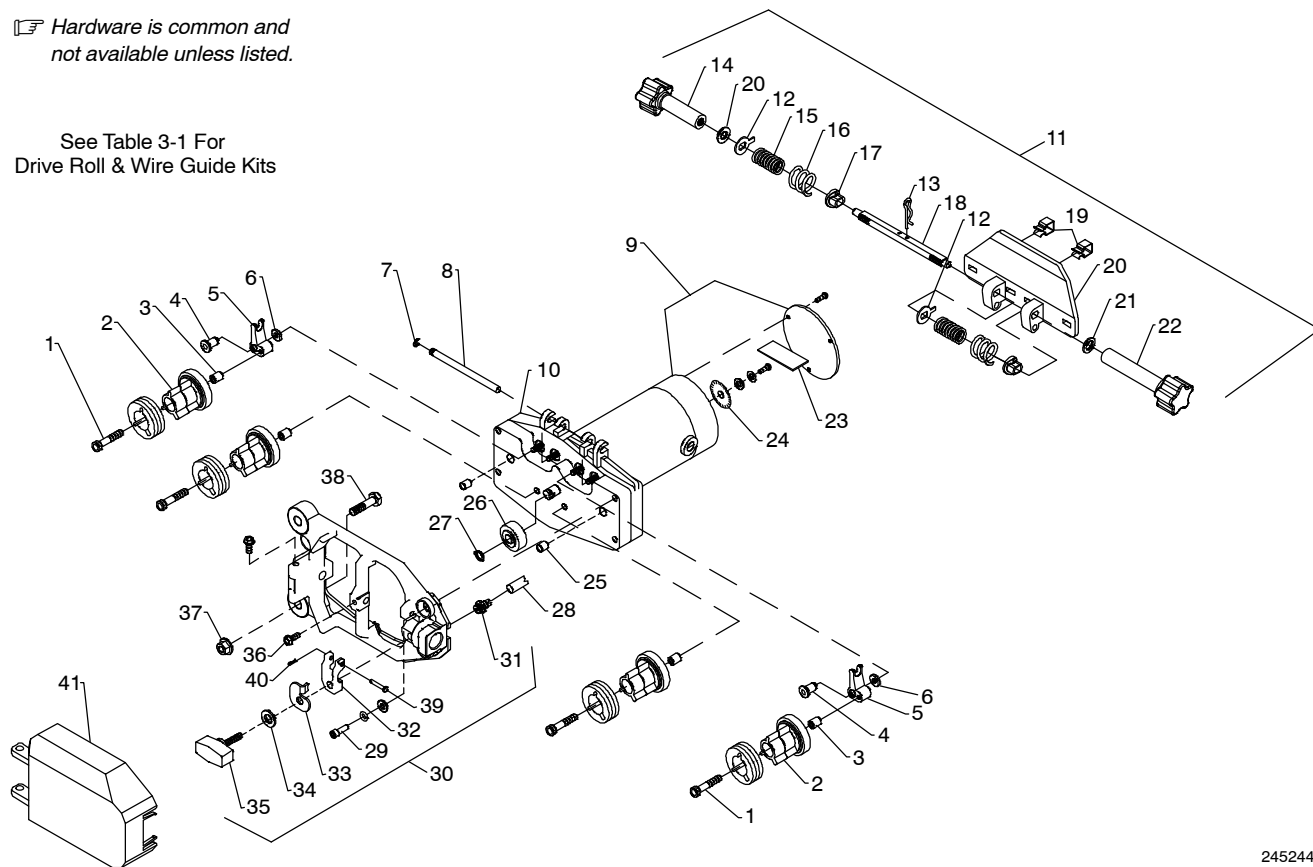
Figure 3-3. Drive Assembly, Wire
