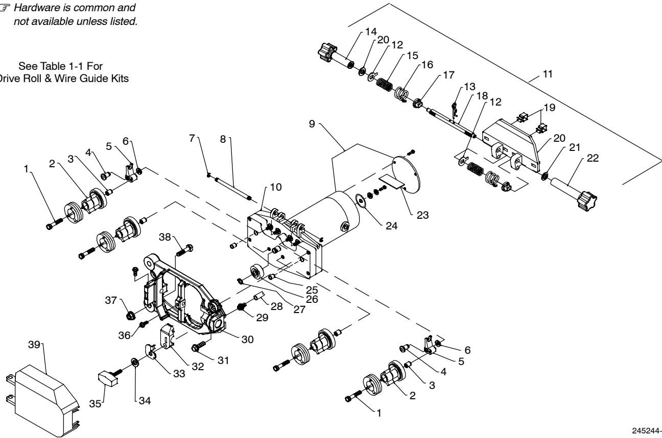
Figure 1-3. Drive Assembly, Wire
